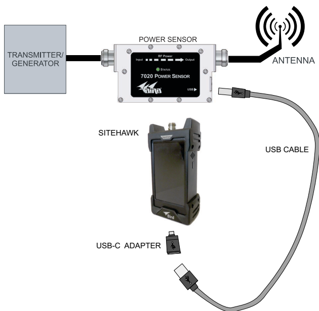
Figure 2 SiteHawk - Power Sensor Connections
